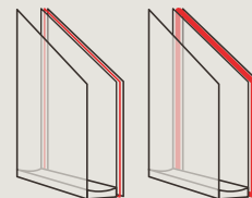
Laminated safety glass (LSG) with four PVB film layers for impact-resistant Class P4A glazing in accordance with DIN EN 356
